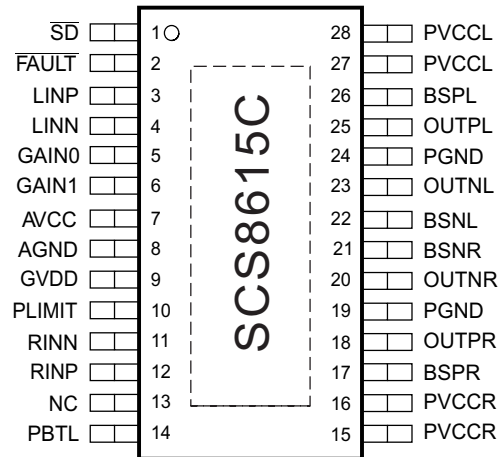
(TSSOP28-PP)PACKAGE (TOPVIEW)
